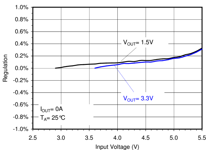
Line Regulation
