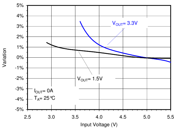
Line Regulation
