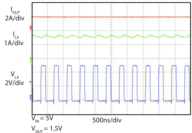
Steady State (PWM) Operation ( I_{OUT} = 2\text{A} )
