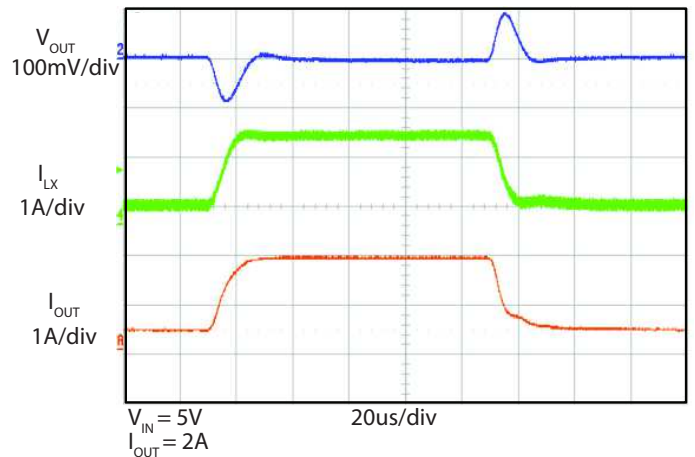
Transient Response ( V_{out}=3.3V , I_{out}=0.4A to 2A )
