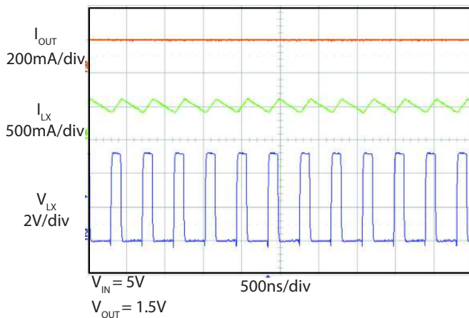
Steady State (PWM) Operation ( I_{OUT} = 200\text{mA} )
