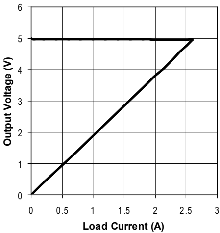
Load Characteristic
