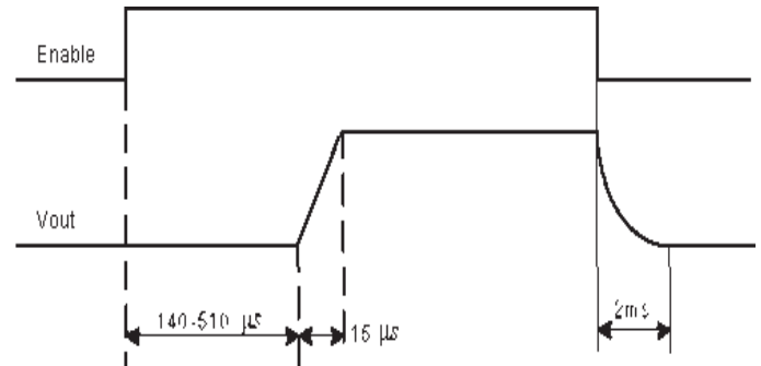
Figure 1: Timing Diagram
