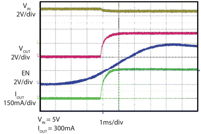
Start Up (Enable) ( V_{OUT}=3.3V )
