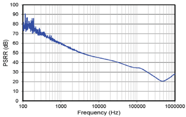
V_{OUT}=1.8V, \text{PSRR}, I_{OUT}=30\text{mA}
