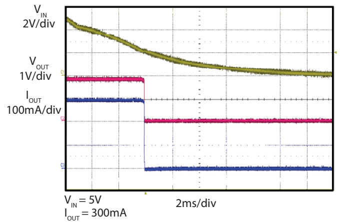
Shutdown ( V_{OUT}=1.8V )
