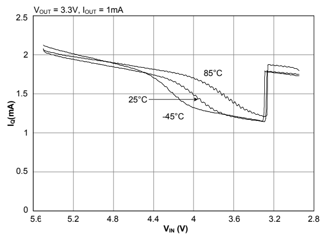
Quiescent Current
