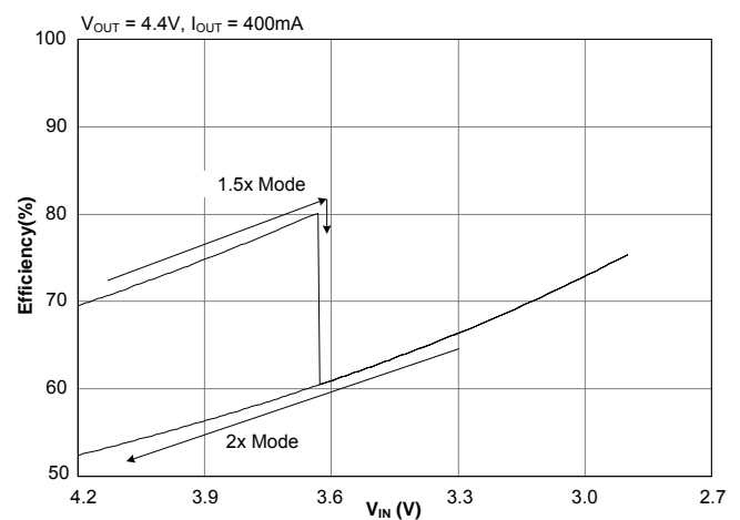
Efficiency — 400mA
