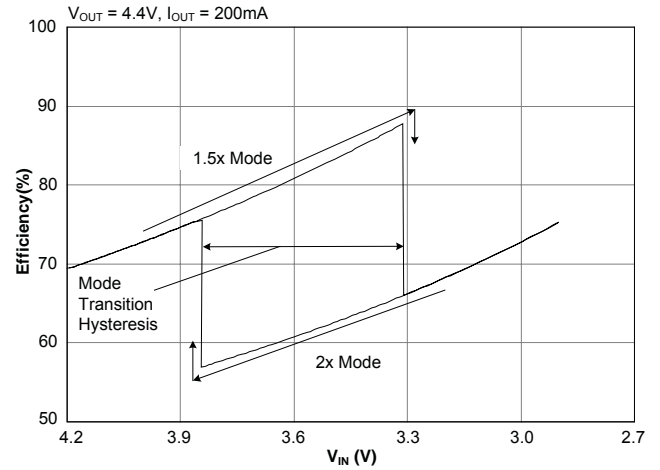
Efficiency — 200mA
