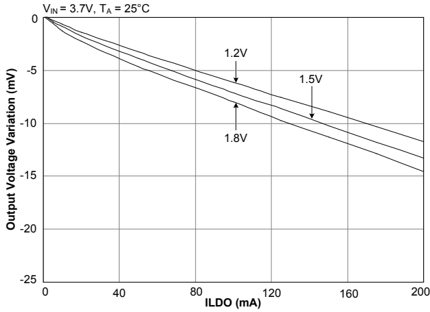
Load Regulation (LDO2)
