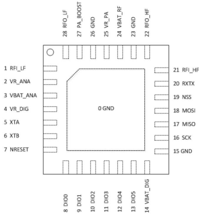
Figure 2. Pin Diagram
