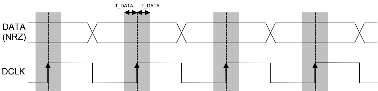
Figure 21. Tx Processing in Continuous Mode
