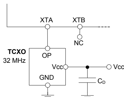
Figure 30. TCXO Connection
