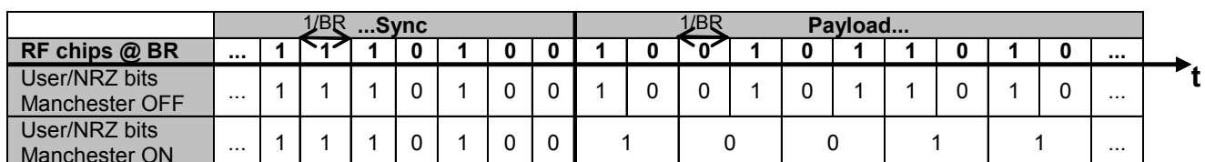
Figure 27. Manchester Encoding/Decoding
