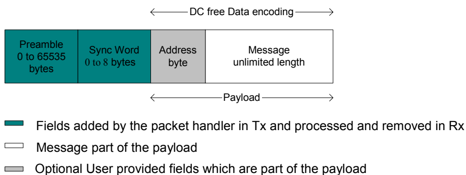
Figure 26. Unlimited Length Packet Format
