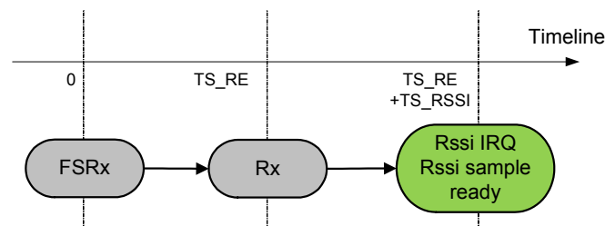
Figure 9. Time to RSSI Sample
