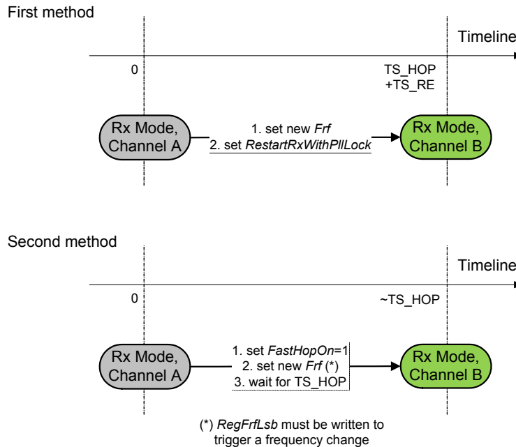
Figure 12. Receiver Hopping
