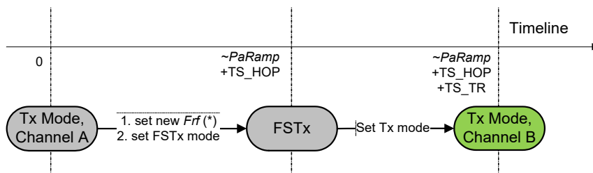
Figure 23. Transmitter Hopping
