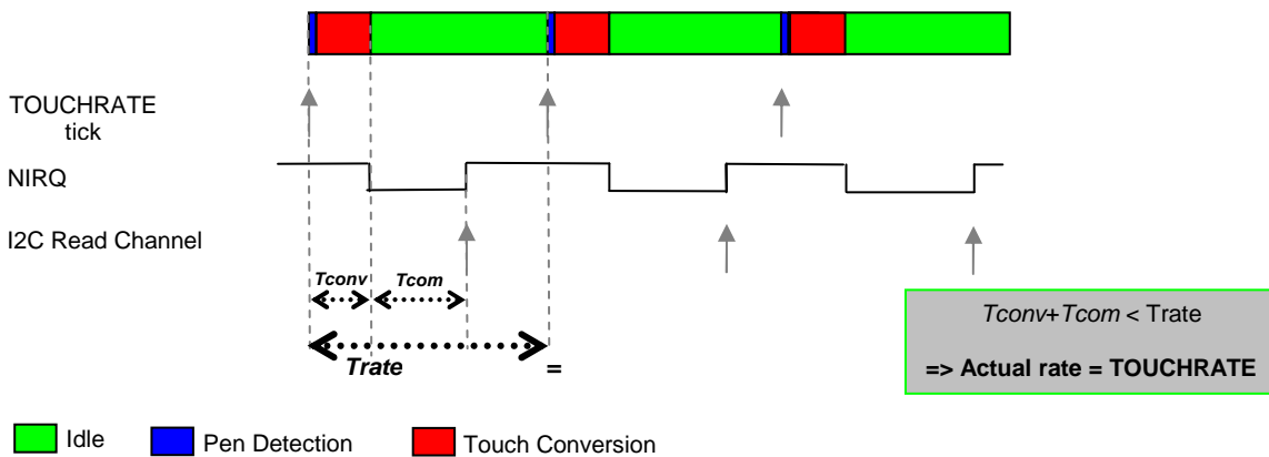
Figure 22 – Correct TOUCHRATE setting
