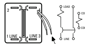
Two Pole (1 pole relay)
