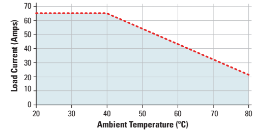
HS072 w/90 Amps single channel SSR
