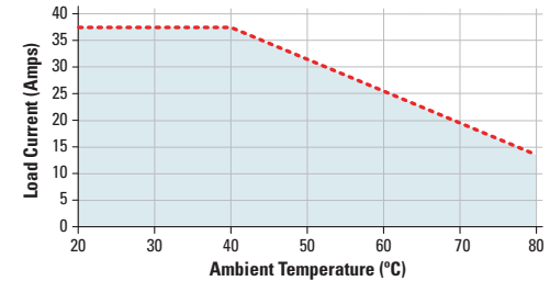
HS172 w/50 Amps single channel SSR
