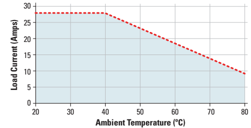
HS251 w/50 Amps single channel SSR
