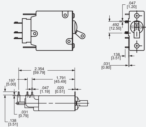
Printed Circuit Board Mounting Terminal Type "R"
