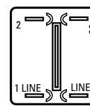
Two Pole (1 pole relay)
