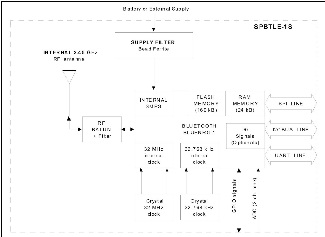
Figure 3 - BLUENRG-M2SA, Block Diagram
