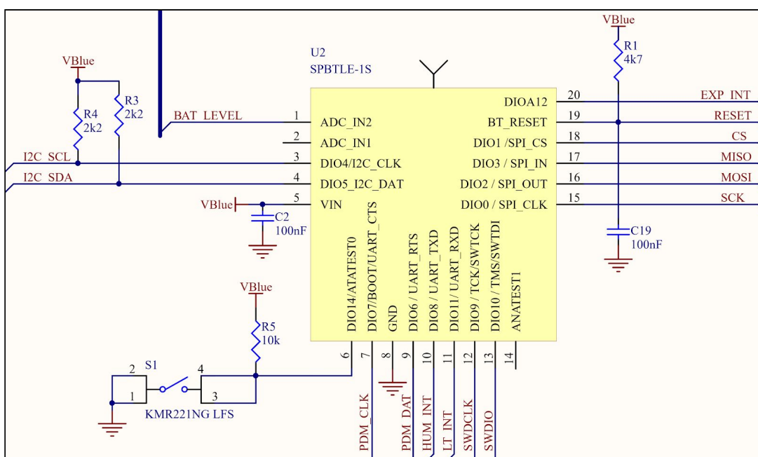
Figure 4 - BLUENRG-M2SA, Schematic Connections
