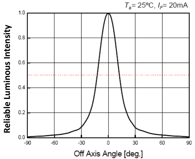
Directivity
