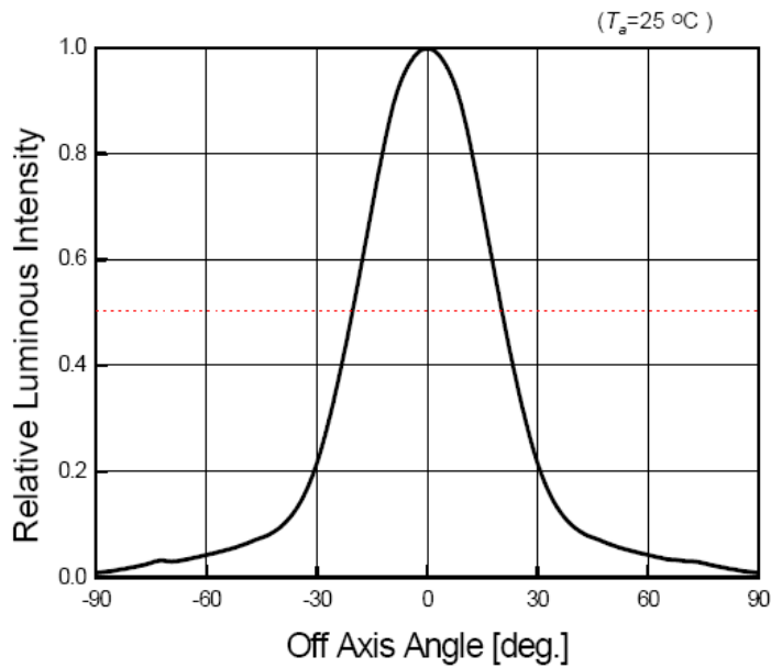
Radiation Diagram
