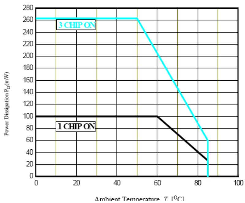
Ambient Temperature vs. Power Dissipation
