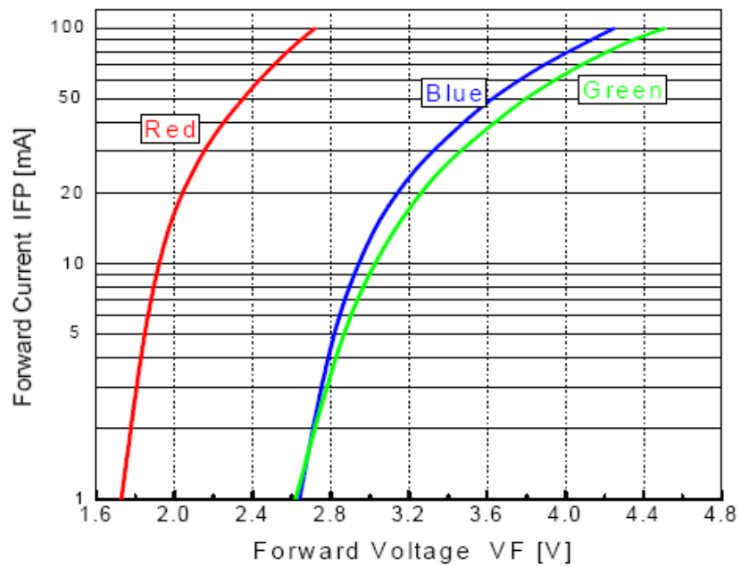
Forward Current vs. Forward Voltage (per die) ( T_a=25\text{ }^\circ\text{C} )
