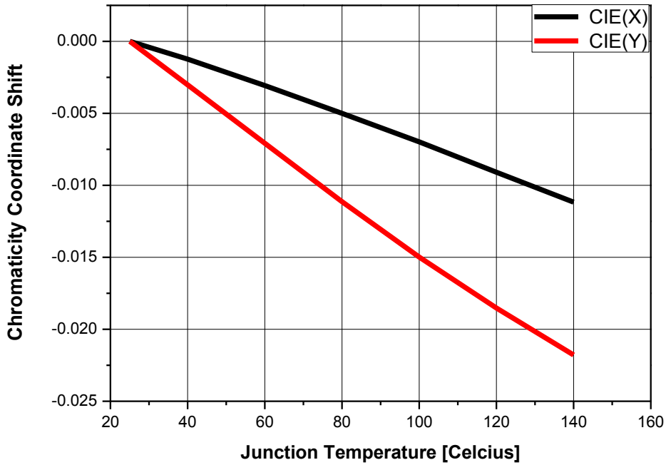
Fig 7. Junction Temperature vs. Chromaticity Coordinate , IF=350mA
