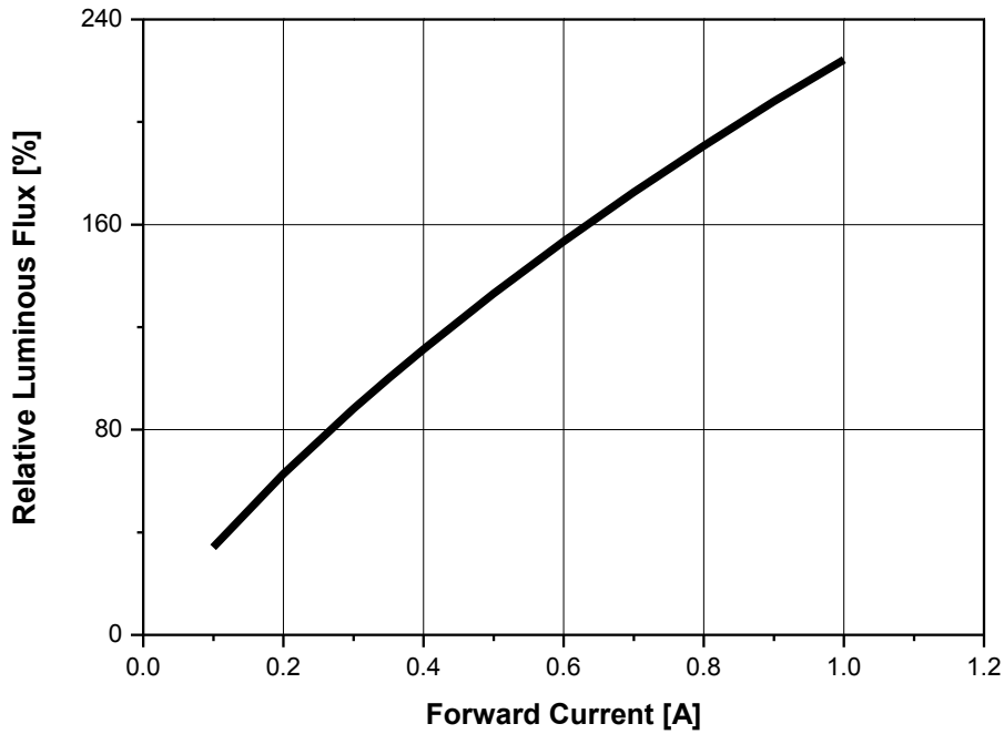
Fig 3. Forward Current vs. Normalized Relative Luminous Flux, Ta=25°C.
