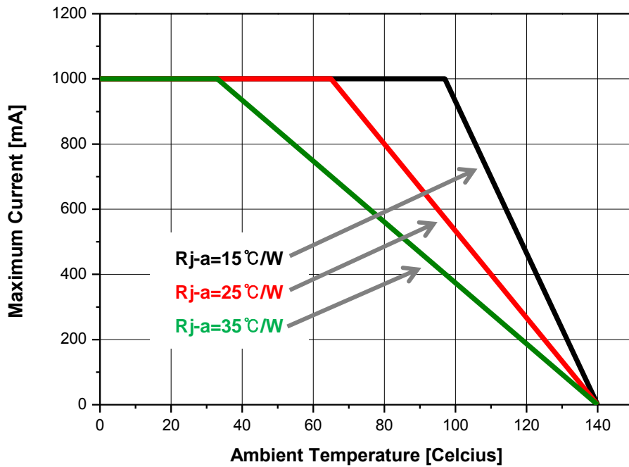
Fig 10. Ambient Temperature vs. Allowable Forward Current ( T_j \text{ max} = 145^\circ\text{C} , @1A)
