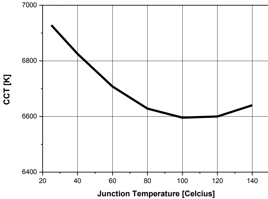
Fig 9. Junction Temperature vs. CCT, IF=350mA
