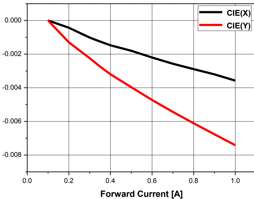
Fig 4. Forward Current vs. Chromaticity Coordinate, Ta=25°C
