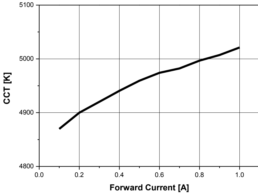
Fig 5. Forward Current vs. CCT, Ta=25°C
