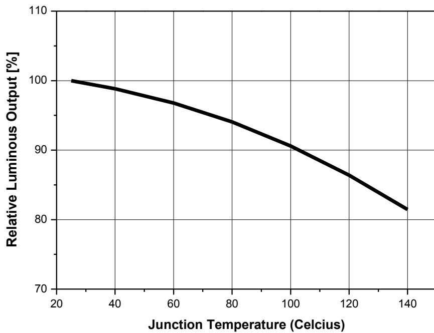
Fig 6. Junction Temperature vs. Relative Light Output , IF=350mA
