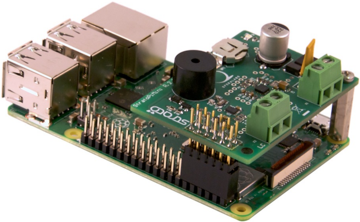
STRATO PI MINI BOARD INSTALLED ON THE RASPBERRY PI
