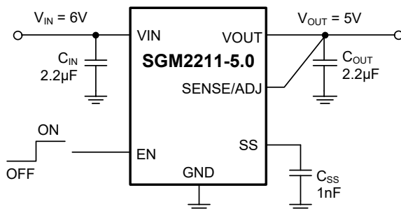
Figure 1. SGM2211 with Fixed Output Voltage, 5V (TDFN-2×2-6AL)
