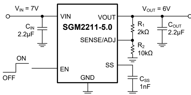
Figure 2. SGM2211 with 5V Output Adjusted to 6V (TDFN-2×2-6AL)
