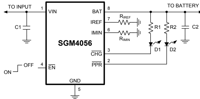
Figure 1. Typical Application Circuit Interfacing to Indication LEDs
