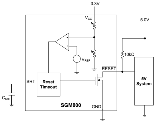
Figure 1. Open-Drain RESET Output Allows Use with Multiple Supplies
