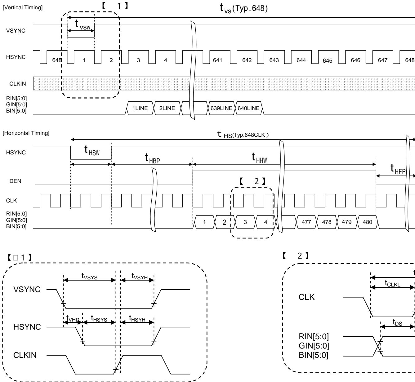
Fig 7-3 LCDIF signal timing in Portrait VGA mode
