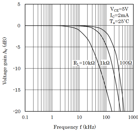
Fig.15 Frequency Response
