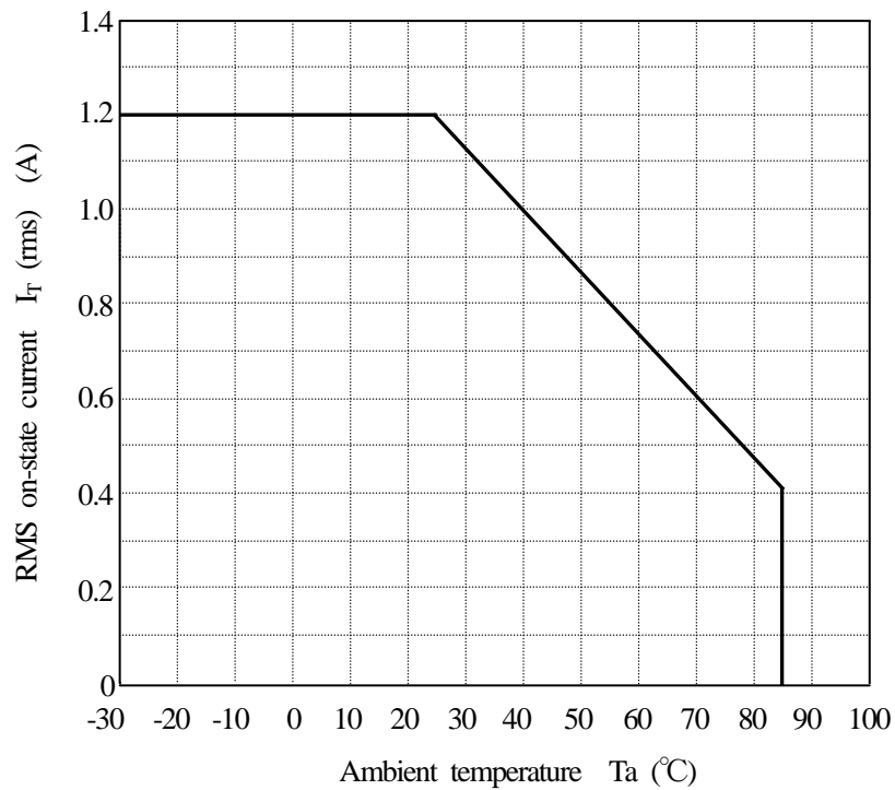
Fig.2 RMS on-state current vs. ambient temperature(*1)
