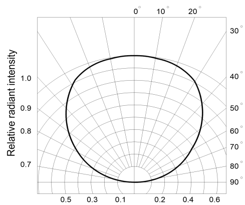
Fig.6 Radiation diagram
