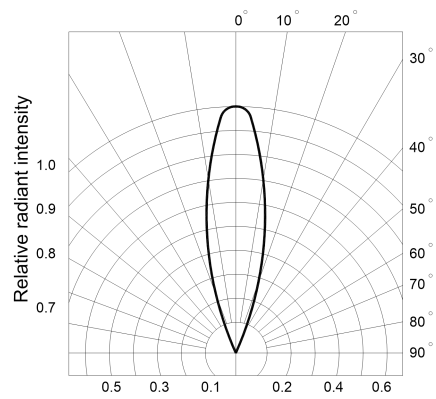
Fig.6 Radiation diagram
