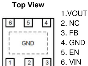
WDFN2020-6L
