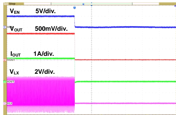
Figure 15. Power Off through EN Waveform
