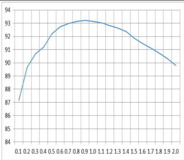
The efficiency for VOUT=5V
