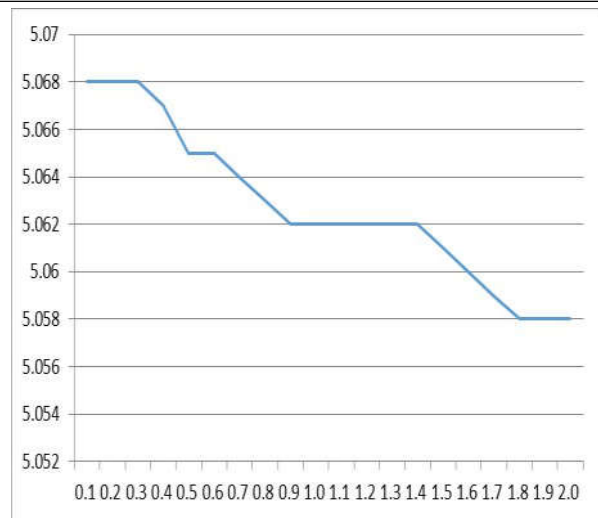
The Load Regulation for VOUT=5V
