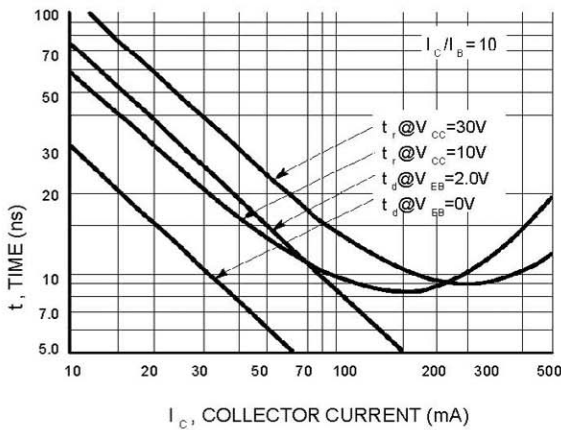
Figure 5. Turn-On Time
