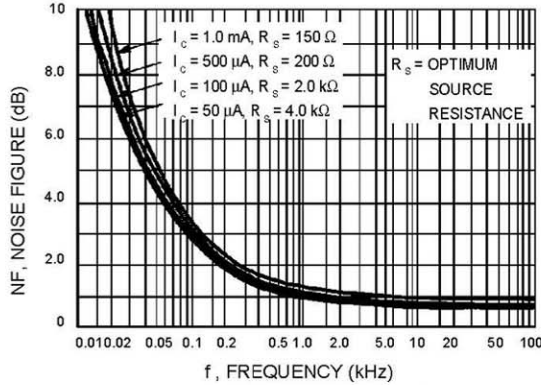
Figure 9. Frequency Effects
