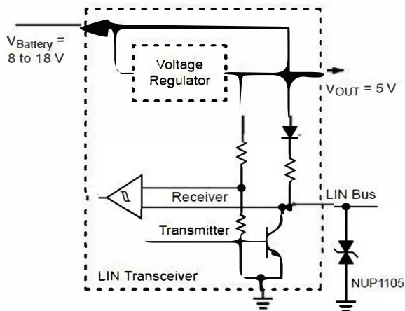
Figure 6. LIN Transceiver
