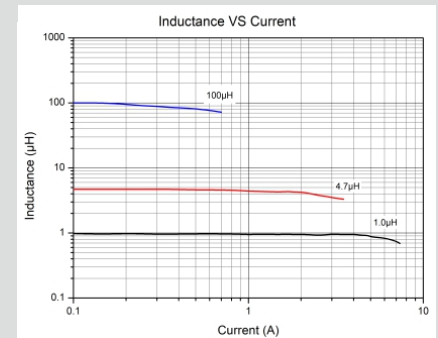
SKNR5040 TYPE
