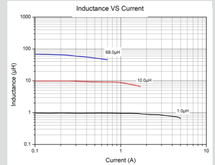
SKNR4020 TYPE
