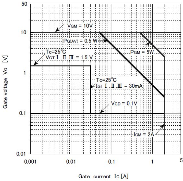
Gate characteristic
