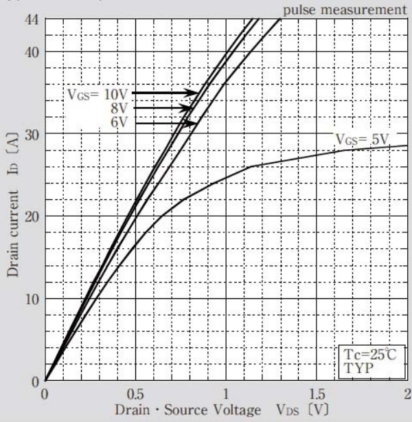
Typical Output Characteristics
