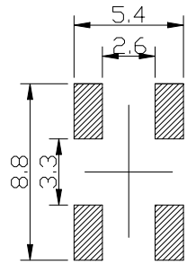
PCB. 焊接图 PCB. WELDING DRAWING
