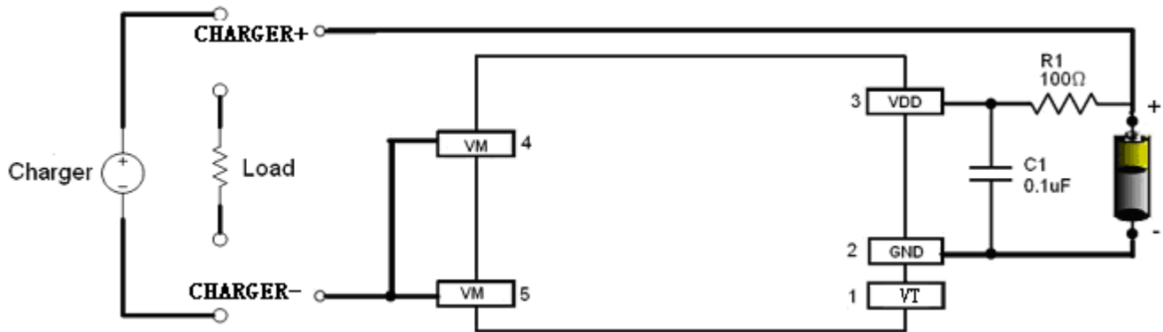
Fig 6 SD5350A in a Typical Battery Protection Circuit
