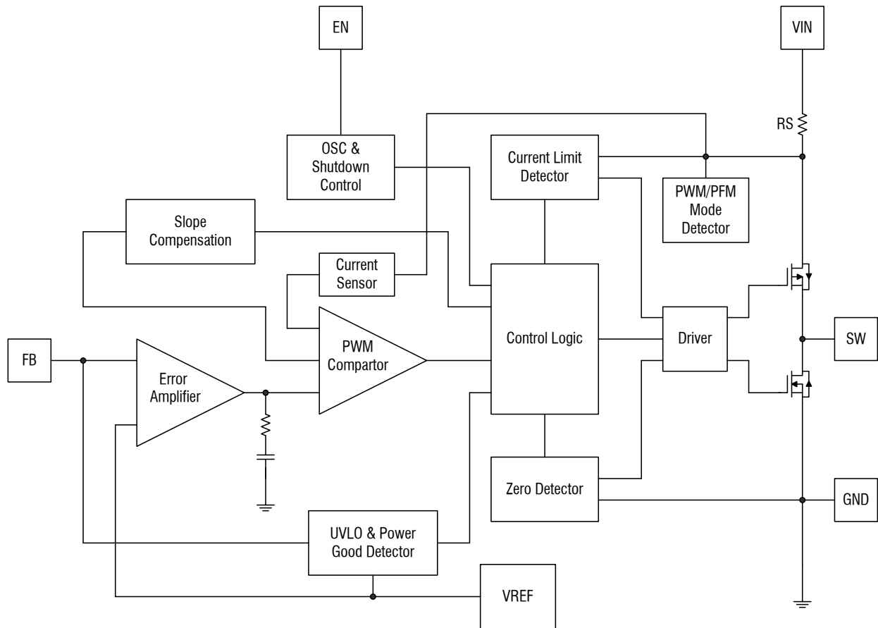
Figure 2. SD8916A Block Diagram
