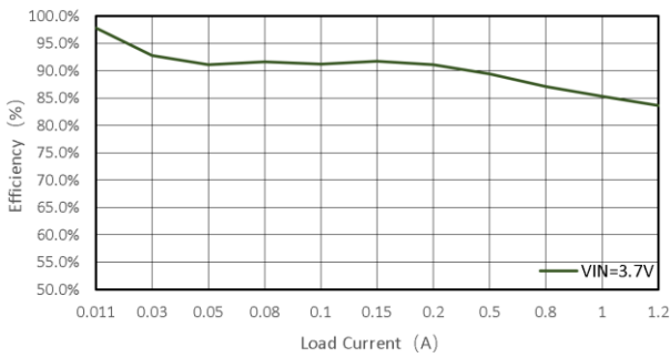
Efficiency @ Vout=5V
