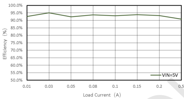
Efficiency @ Vout=12V
