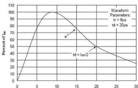
Pulse Waveform
