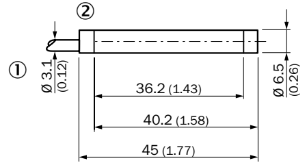
Standard-body, non-flush, cable
