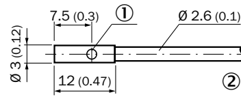
Ultrashort, flush, cable
