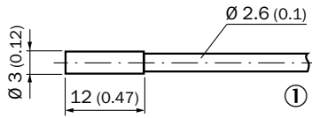
Ultrashort, flush, cable, IHPO3
