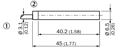
Standard-body, flush, cable
