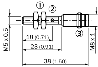
Standard-body, flush, connector
