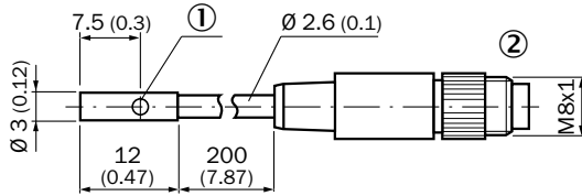
Ultrashort, flush, cable with connector
