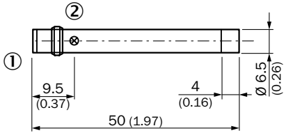
Standard-body, non-flush, connector
