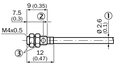
Ultrashort, flush, cable
