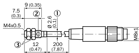
Ultrashort, flush, cable with connector
