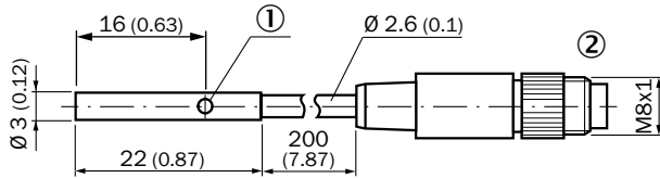
Standard-body, non-flush, cable with connector, with knurled nuts
