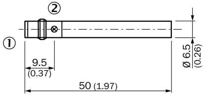
Standard-body, flush, connector
