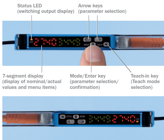
Ensures comfortable reading: for difficult installation conditions, the 7-segment display can be inverted.
