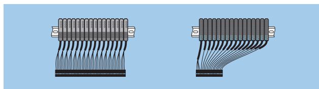
Simple calculation: 64 terminals will be required without Wire Saving (shown on left), only 34 terminals with Wire Saving (shown on right).
