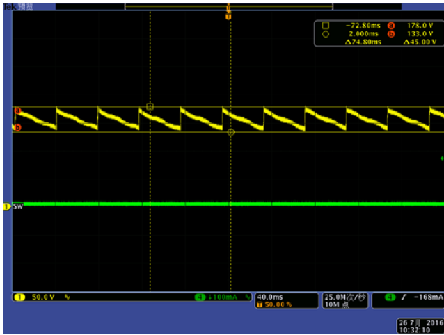
176Vac CH1:Vo
