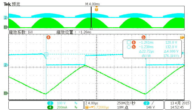
CH3:Vds CH4:Ics
