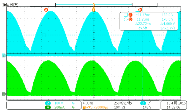
CH3:Vds CH4:Ics
