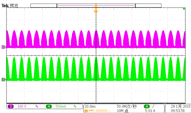
CH3:Vds CH4:Ics
