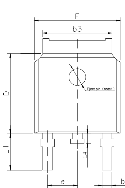
TO-252-2L
