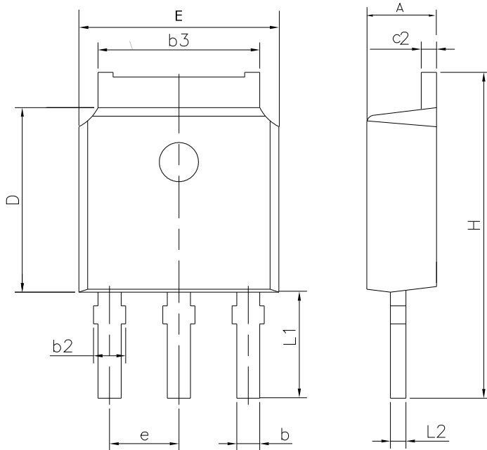
TO-251J-3L
