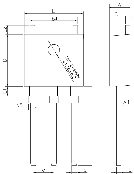
TO-251J-3L
