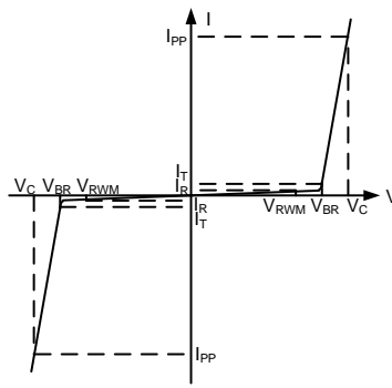
Figure 1. Bi-directional TVS
