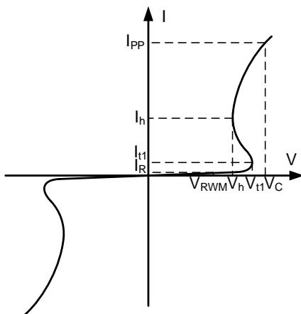
Figure 1. Bi-Directional TVS
